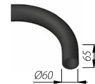
spigot ending of the arm
