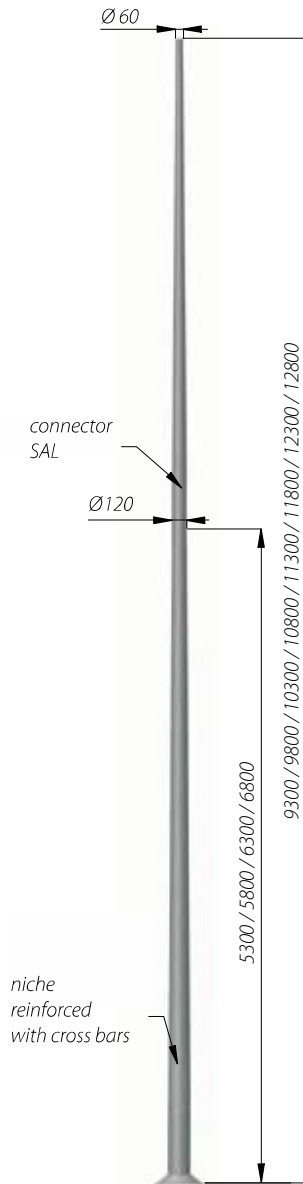
Columns with base plate
