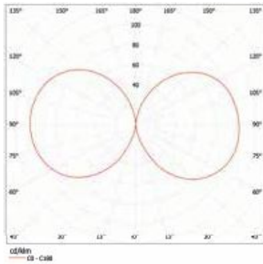
Distribution curve for SAL DECO-3 LED
